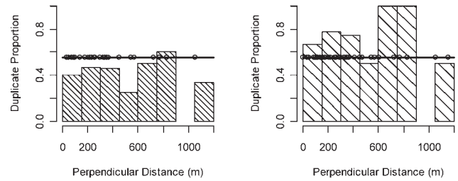
Proportion of Observer 1 detections seen by Observer 2 Proportion of Observer 2 detections seen by Observer 1
