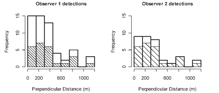
Proportion of Observer 1 detections seen by Observer 2 Proportion of Observer 2 detections seen by Observer 1
