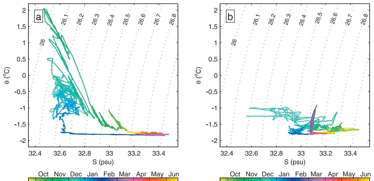
Figure 7. Scatterplots of bottom water properties at (a) inshore mooring and (b) offshore moorings, color-coded with time. Dashed lines are isopycnal ( \sigma_{\theta} = \text{const} ) contours (labeled in \text{kg m}^{-3} ).
