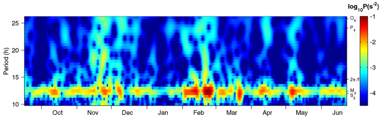
Figure 14. Distribution of vertical shear variance as a function of time and period (clockwise-rotating). Data from 40 m off the bottom at the inshore mooring are shown. Periods of major tidal constituents as well as the inertial period ( 2\pi/f ) are marked on the right. Rotary wavelet transform with Morlet wavelet of order c = 20 was used.
