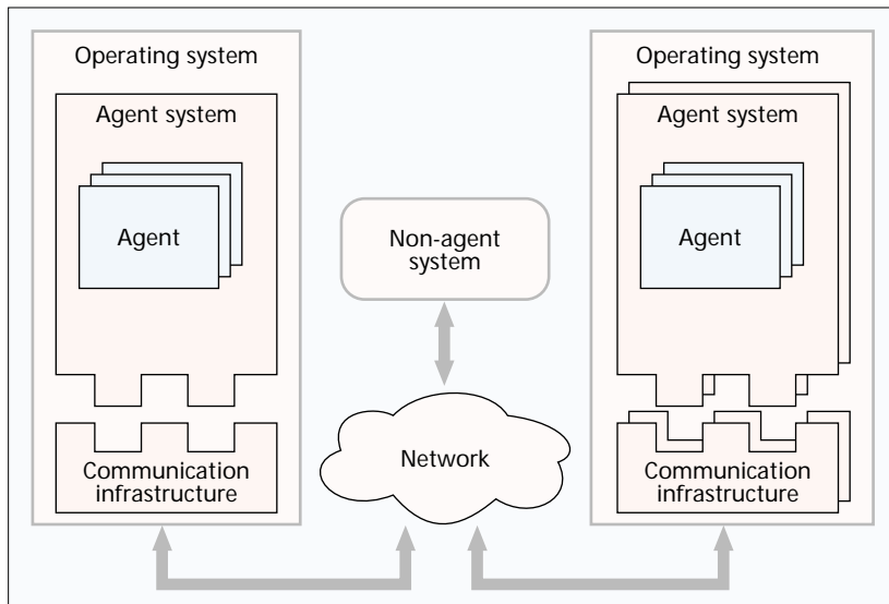
■ Figure 1. Mobile agent facility architecture.
