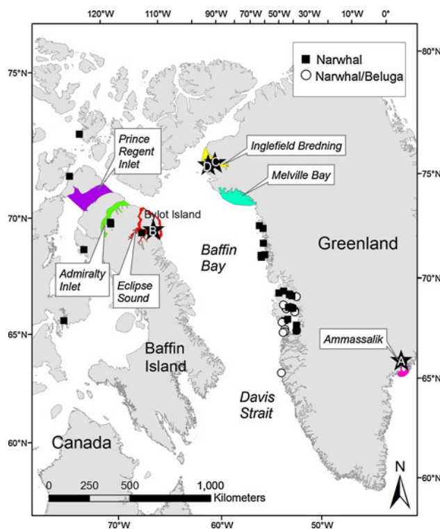
Fig. 1 Map of all reported narwhal sea ice entrapments in Canada and Greenland (1912–2010). Some ice entrapments were comprised of both narwhals and belugas. Stars indicate locations of the four recent sea ice entrapments discussed in this paper (labeled A, B, C, and D). The six narwhal summering areas used for sea ice analyses are shown in different colors
