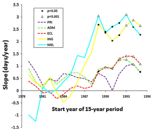
Fig. 3 Slopes of sliding 15-year least-squares fits for western and eastern Baffin Bay narwhal summering areas. The slope of the least squares line is plotted for each 15-year period. Canadian summering areas are shown as dashed lines
