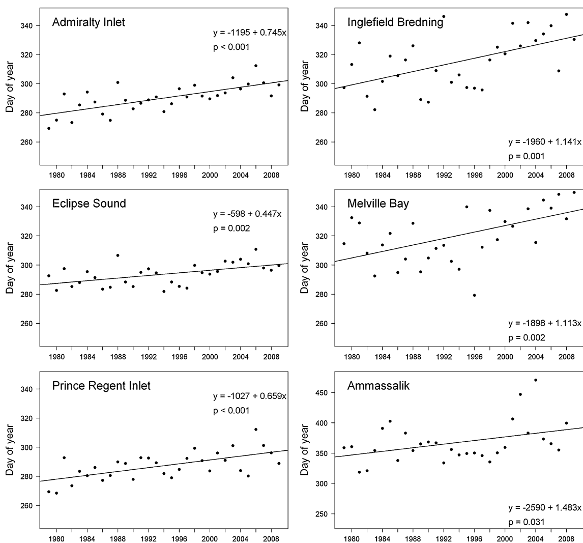
Fig. 2 Time series of the day of year of autumn freeze-up in narwhal summering areas (1979–2009), derived from the 65% threshold of sea ice concentration (Ammassalik 45% threshold). All trends are significant at P < 0.05 and insensitive to choice of threshold
