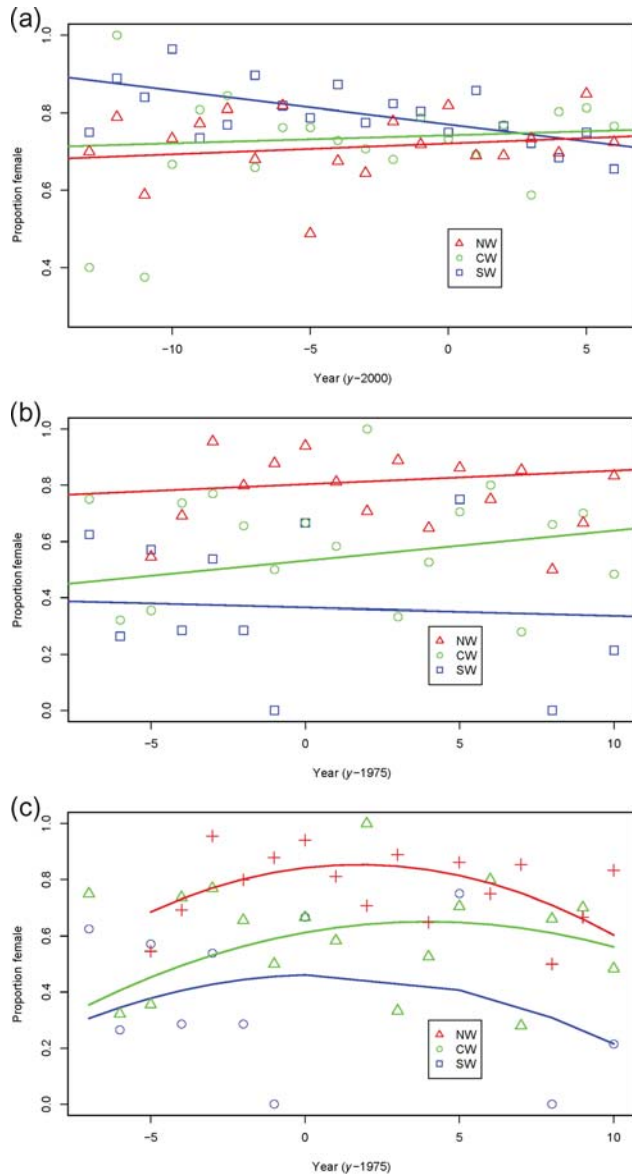
Figure 5. Linear model fits to the proportion of females in (a) the late Greenland catch and (b) the offshore Norwegian catch, and (c) quadratic model fits to the proportion of females in the Norwegian offshore catch in each of the three regions. The proportion of females was weighted by sample size for each region and year to characterize graphically the trends in the data.
