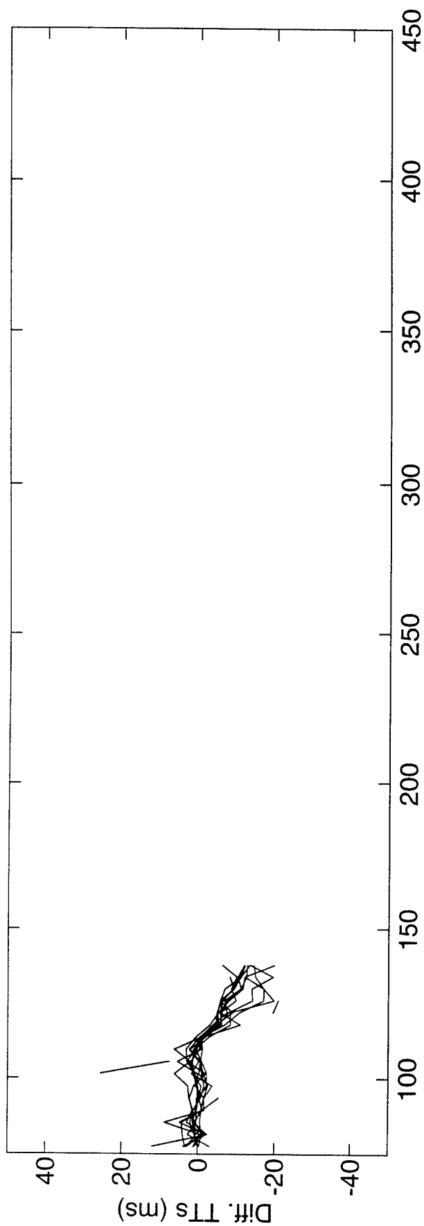
Differential Travel Times 5a<=>6
