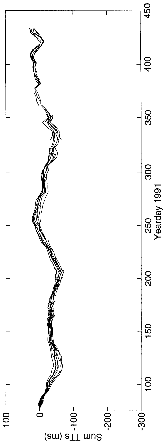
Sum Travel Times 3 \leq \leq 6
