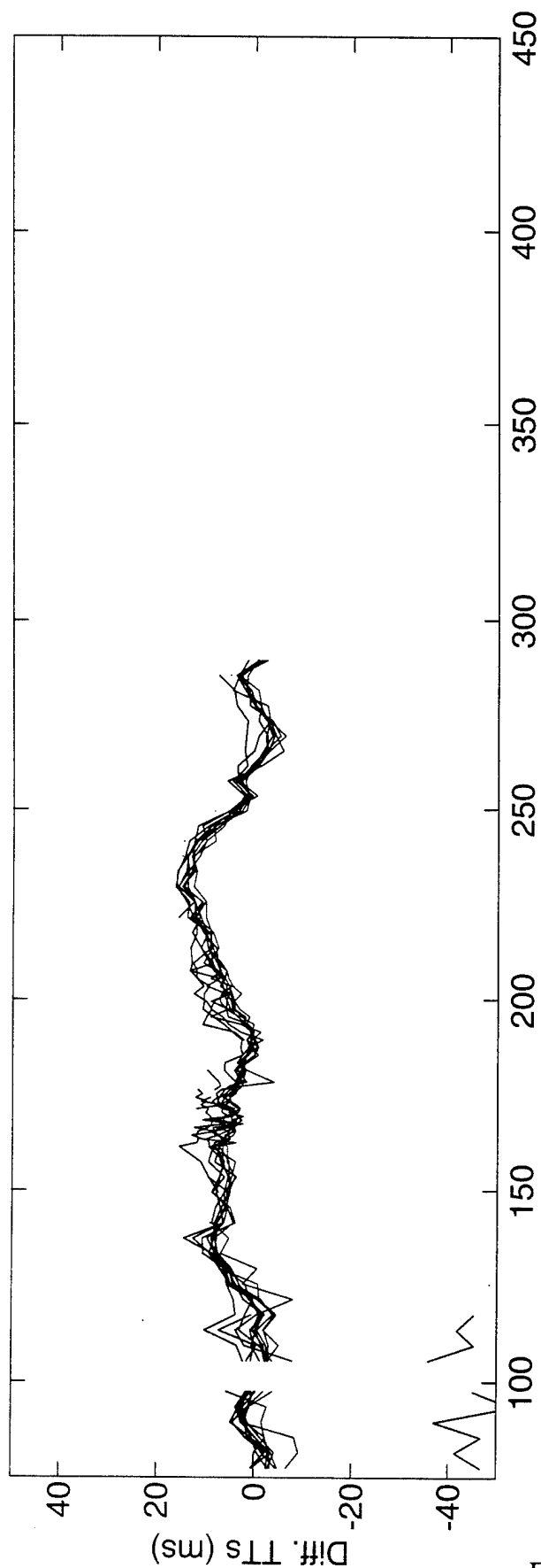
Differential Travel Times 4<=>6
