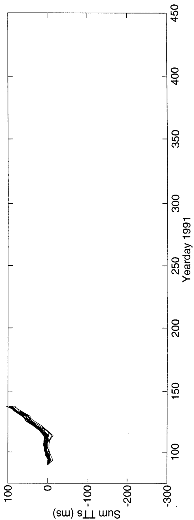
Sum Travel Times 2<=>5a
