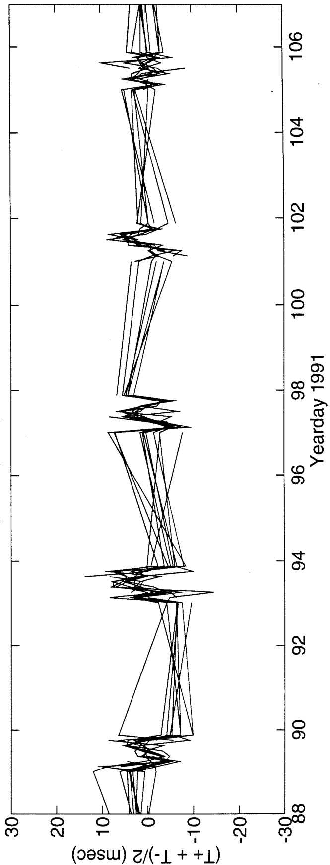
DeTided High Frequency Sum Travel Times 1 \leq \leq 6
