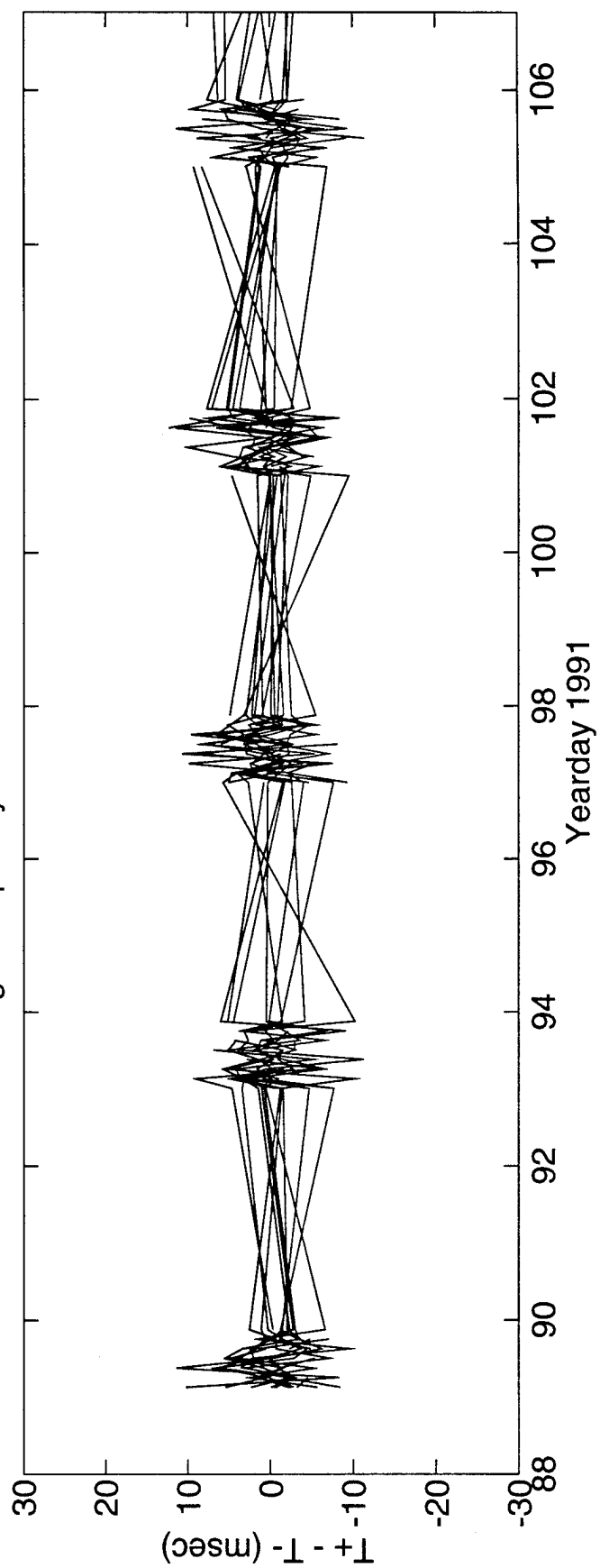
DeTided High Frequency Difference Travel Times 2<=>5a
