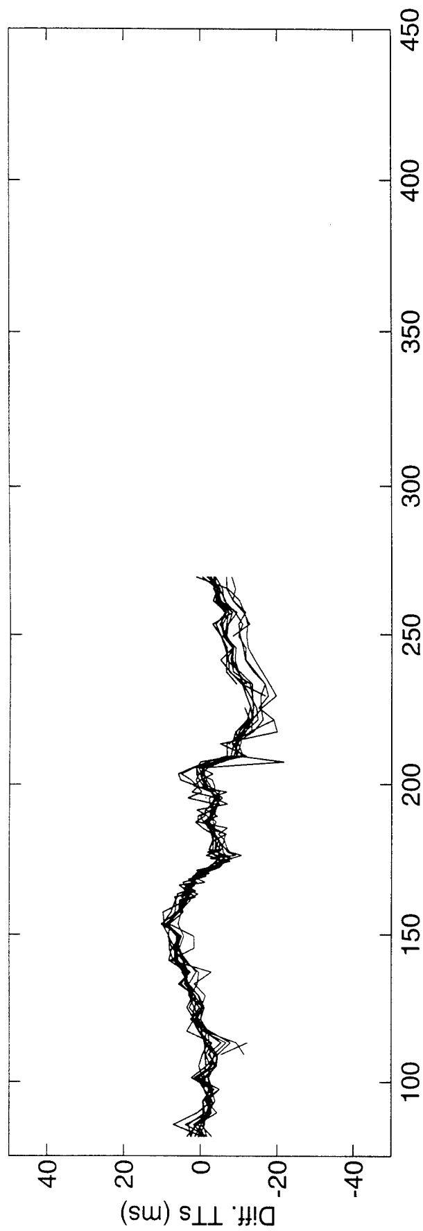
Differential Travel Times 1 \leq 6
