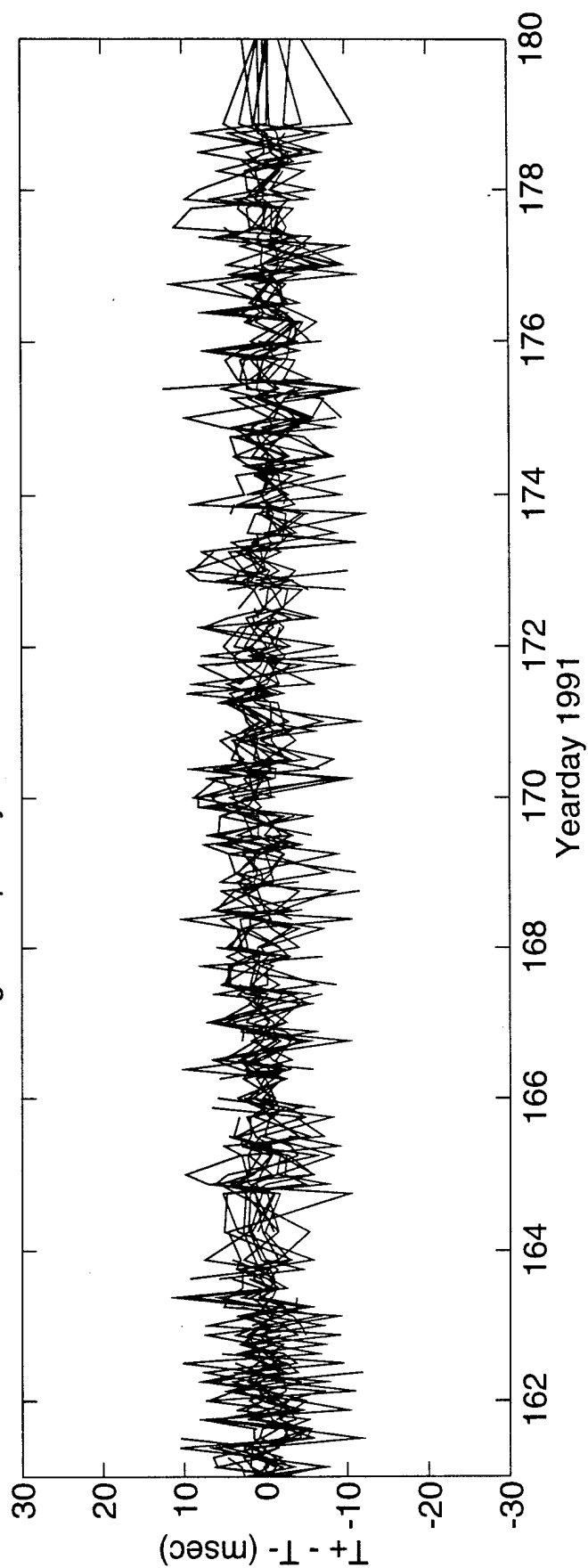
DeTided High Frequency Difference Travel Times 1 \leq 3
