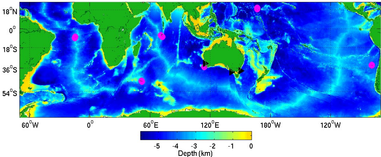
Figure 3. The locations of existing CTBTO hydrophone stations (magenta circles) and the regional Australian hydrophone facilities (black triangles), together with ocean bathymetry derived from the Smith-Sandwell atlas. Each CTBTO receiver consists of a triplet of hydrophones for directionality. Data are recorded, processed, and shipped to shore in real time from these arrays.
