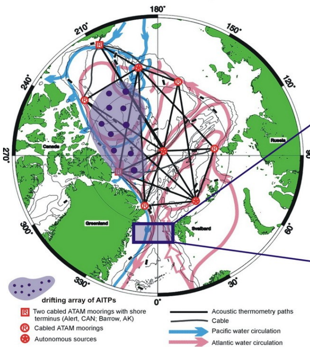
Figure 5. The envisioned basin-wide AURORA mooring grid in the Arctic Ocean (left panel) and the existing moored observatory in Fram Strait (right panels). In addition to moored instrumentation, an array of drifting Acoustic Ice Tethered Platforms (AITP) with acoustic modems for communications will be deployed in the Arctic Ocean, while in Fram Strait profiling gliders, capable of under-ice acoustic navigation, will be employed. In the right lower panel, positions of moorings are overlaid on the temperature distribution in Fram Strait, an inflow of the warm Atlantic water in the West Spitsbergen Current depicted by red color (XR: [43]).
