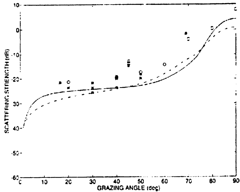
Figure 7. Comparison of backscattering model with data from SAXON FPN. Model inputs are f = 70 kHz; and U = 8 m/s (solid line), and 16 m/s (dashed line). Circles represent data taken in the wind speed interval 12 < U \leq 16 m/s; asterisks represent data taken in the wind speed interval 8 < U \leq 12 m/s.
