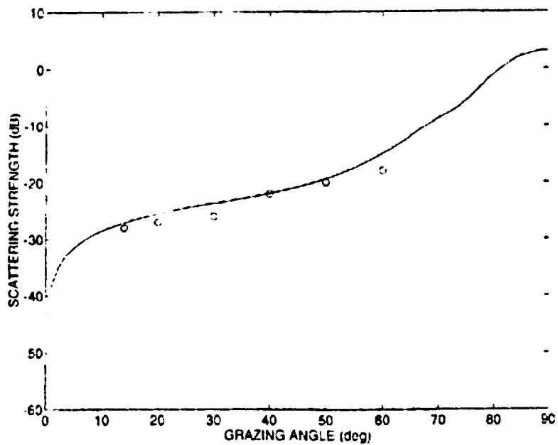
Figure 8. Comparison of backscattering model with data from NOREX85. Model inputs are f = 18 kHz and U = 17 m/s.
