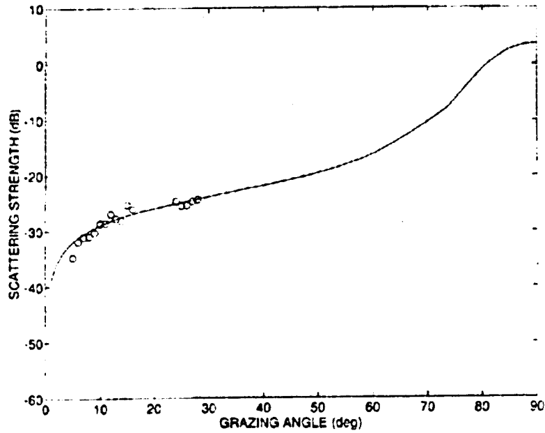
Figure 5. Comparison of backscattering model with data from FLIP77. Model inputs are f = 25 \text{ kHz} and U = 12.8 \text{ m/s} .
