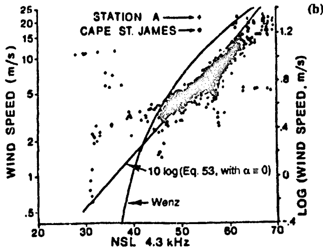
Figure 17. (a) Pressure received at an omnidirectional hydrophone calculated via the Wenz equation, via 10 \log (\text{Eq. 55}) , which does not include bubble effects, and via 10 \log (\text{Eq. 53, with } \alpha \approx 0) , which does include bubble effects. (b) Wenz equation and 10 \log (\text{Eq. 53, with } \alpha \approx 0) compared with data taken by Farmer and Lemon. 52
