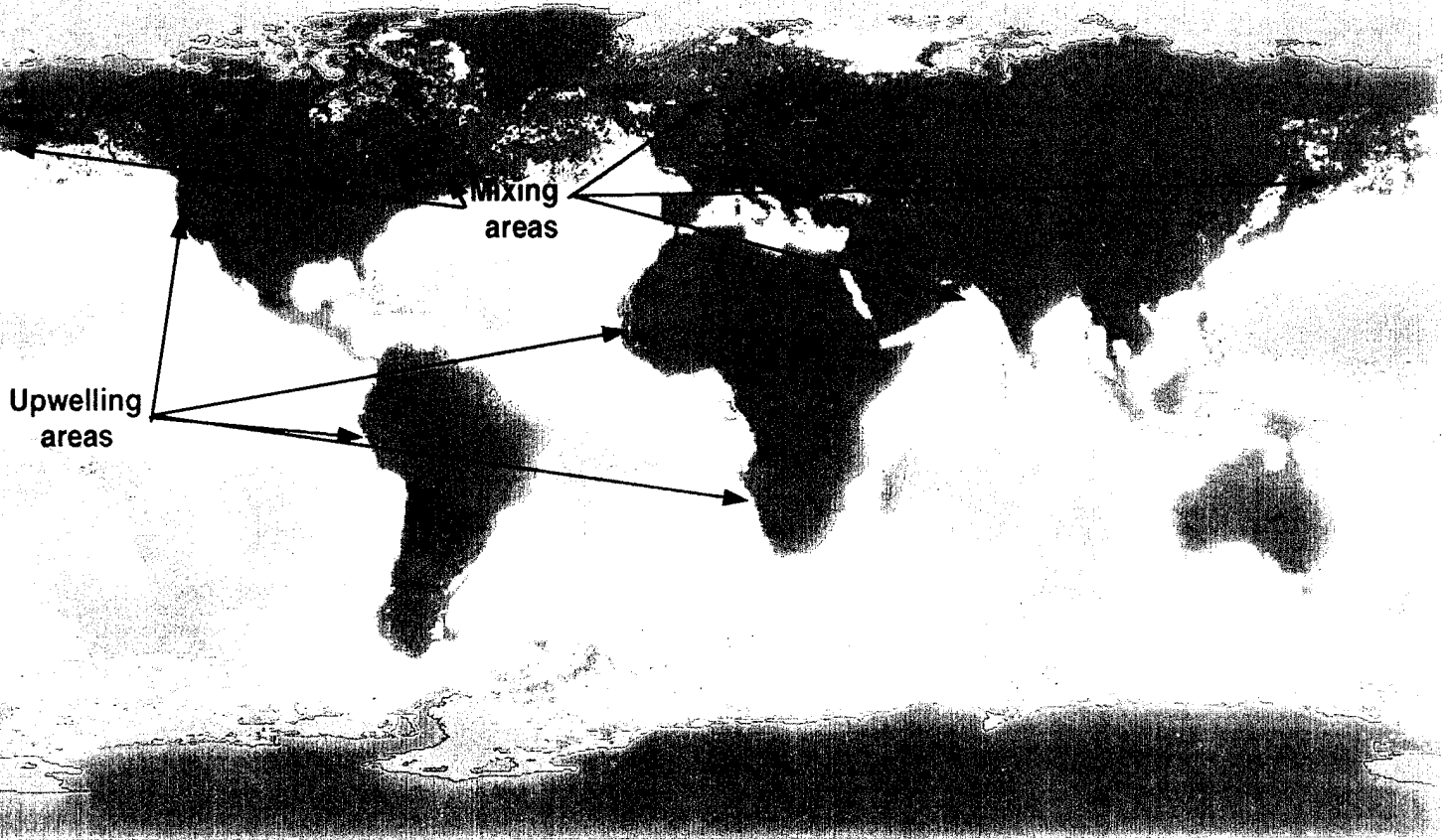
Figure 7. World annual average ocean primary productivity obtained from Coastal Zone Color Scanner satellite images. Major upwelling and front mixing areas are shown. Primary production ranges from orange (low) through yellow and green to blue (high).
