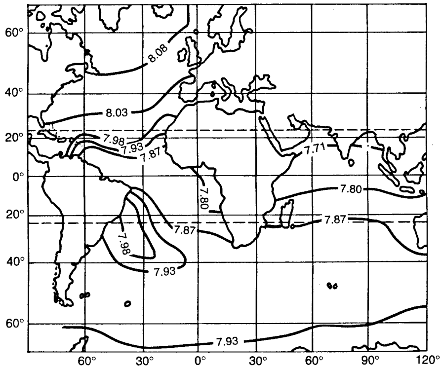
Figure 4. Geographic variation in pH (using contours given by Lovett 17 ).
