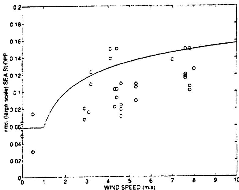
Figure 13. Model for rms sea slope s (equal to square root of Eq. 41a) vs estimates of s derived from measurements of L and inversion of Eq. 40.
