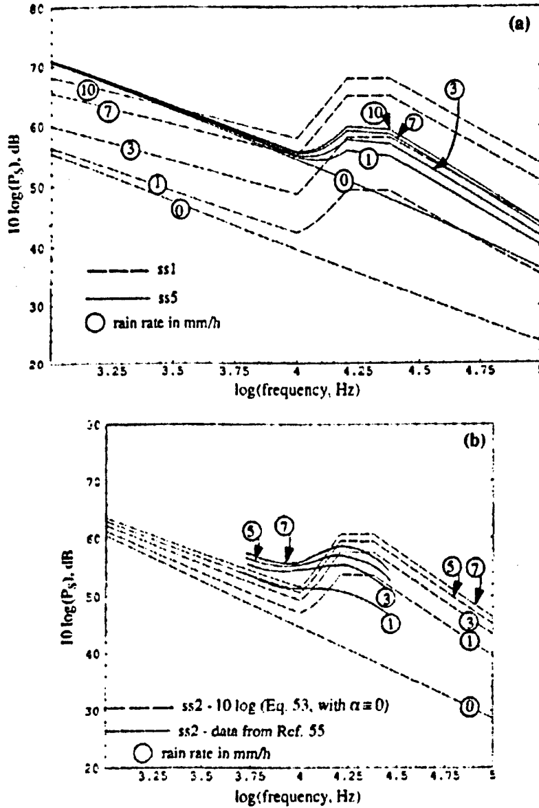
Figure 18. (a) 10 \log (Eq. 53, with \alpha \equiv 0 ) plotted for five rain rates and two sea states. (b) Comparison between 10 \log (Eq. 53, with \alpha \equiv 0 ) and some of the data from Ref. 55.
