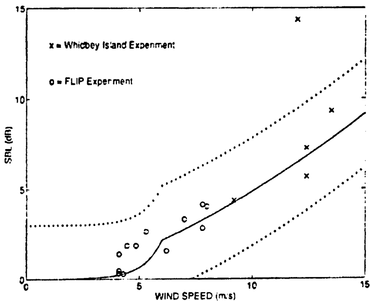
Figure 11. Comparison of SBL model predictions (solid line) with measured 30-kHz data from the FLIP and Whidbey Island experiments. Data from various grazing angles have been normalized to 10° grazing angle. Upper and lower dotted lines represent a \pm 3 dB interval about the predicted curve.
