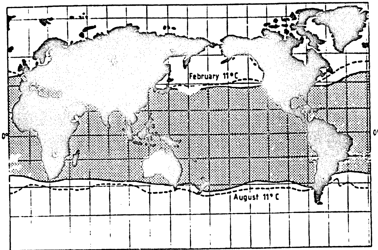
Figure 2. Worldwide distribution of snapping shrimp according to Johnson et al. 2 Snapping shrimp are found in the shaded area wherever the bottom depth is less than 60 m and the bottom sediment is suitable. (after Cato and Bell 3 ).
