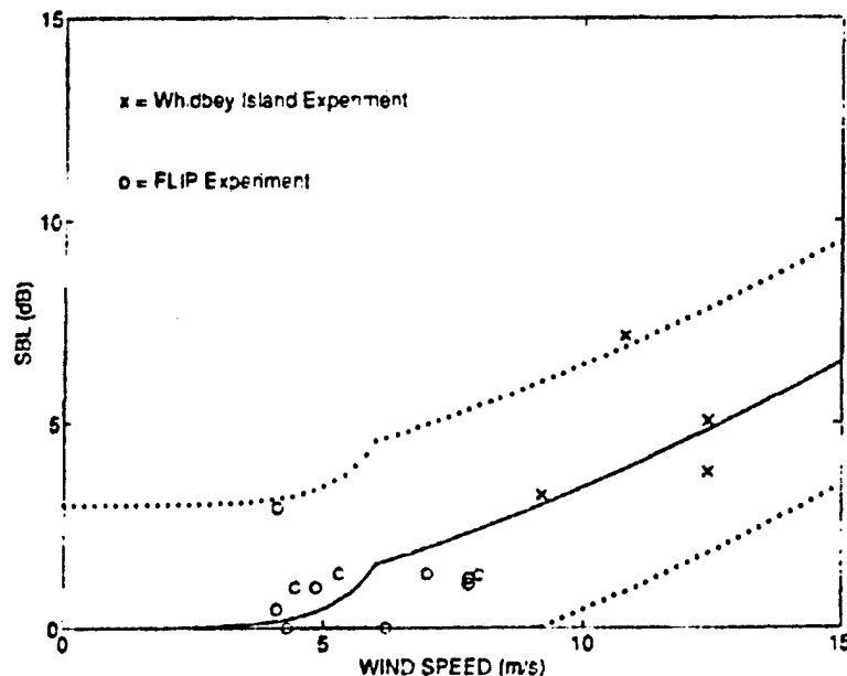
Figure 10. Comparison of SBL model predictions (solid line) with measured 20-kHz data from the FLIP and Whidbey Island experiments. Data from various grazing angles have been normalized to 10^\circ grazing angle. Upper and lower dotted lines represent a \pm 3 dB interval about the predicted curve.
