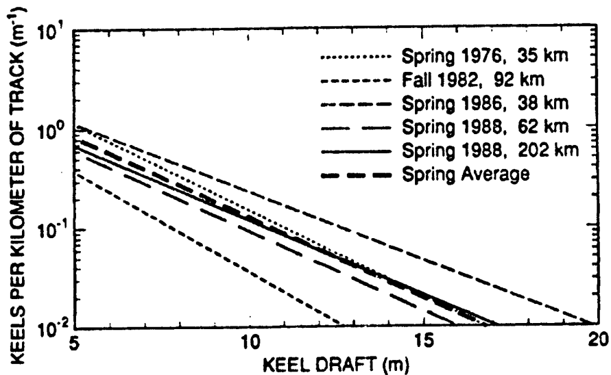
Figure 8. The distribution of maximum drafts of ice keels observed in the under-ice profiles obtained along given tracks of a submarine.
