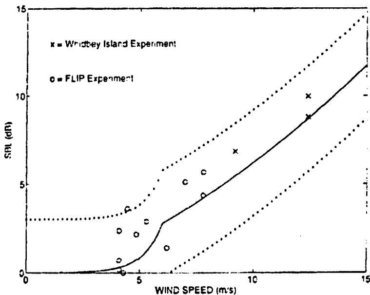
Figure 12. Comparison of SBL model predictions (solid line) with measured 40-kHz data from the FLIP and Whidbey Island experiments. Data from various grazing angles have been normalized to 10° grazing angle. Upper and lower dotted lines represent a \pm 3 dB interval about the predicted curve.
