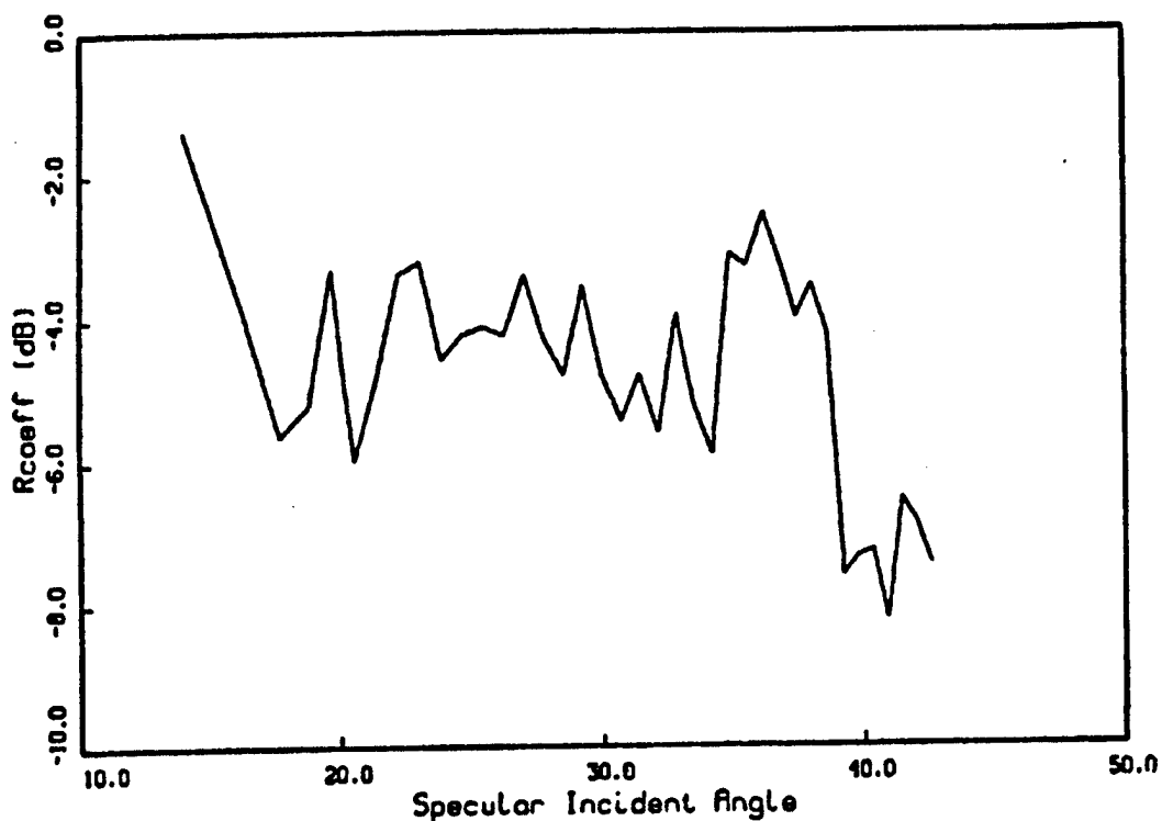
Figure 3. Average of reflection coefficient, R_{coeff} , vs grazing angle for data from Run: 31, 33, and 37 of Ref. 8.
