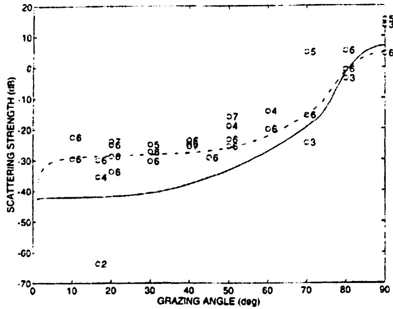
Figure 6. Comparison of backscattering model with data from SAXON FPN. Model inputs are f = 70 \text{ kHz} and U = 1 \text{ m/s} (dotted line), 4 \text{ m/s} (solid line), and 7 \text{ m/s} (dashed line). The number beside each data point is the wind speed.
