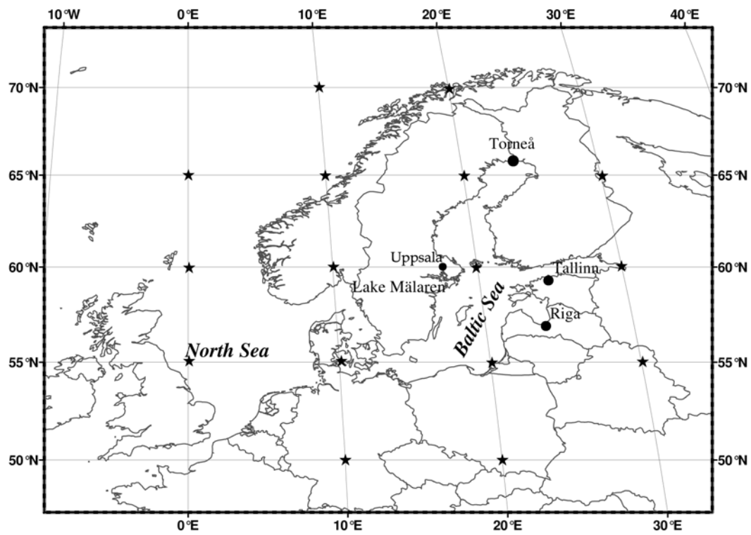
Figure 1 The Baltic Sea and Skagerrak system. Locations of the ice break-up series are indicated with dots. Stars indicate the pressure points used when calculating the atmospheric circulation indices.
