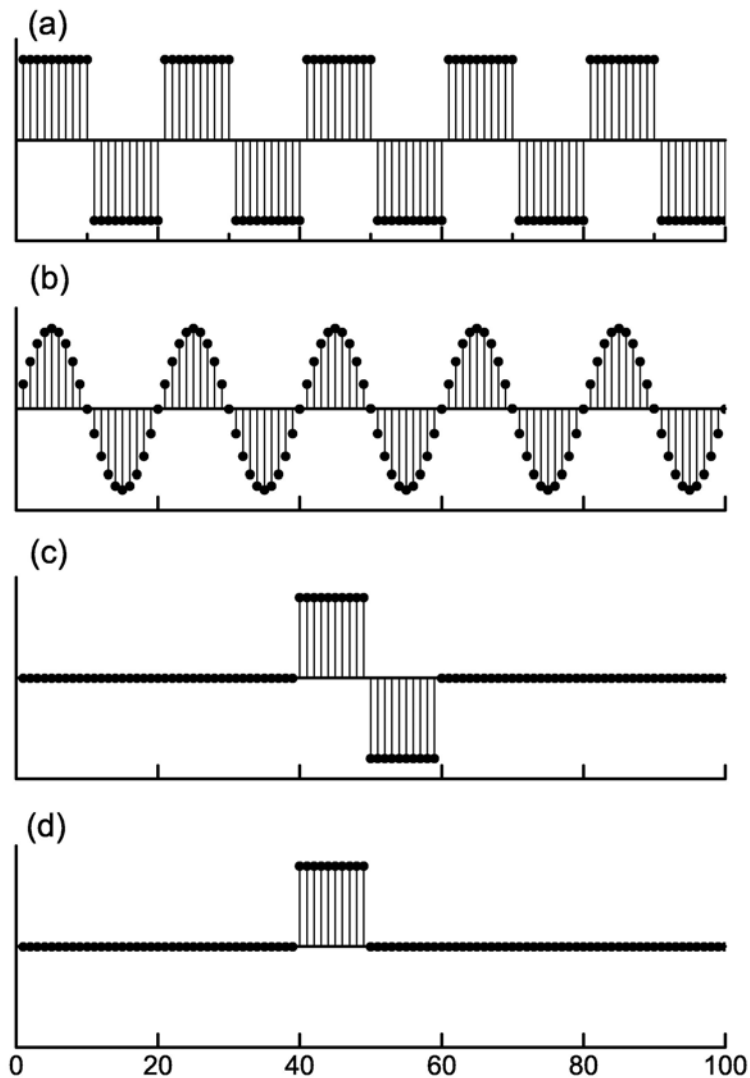
Figure 3 Examples of dictionary elements used in matching pursuits analyses of time series. (a): A vector containing a square wave oscillation with a period of twenty time steps in the time series. (b): A vector containing a sinusoidal oscillation, also with a period of twenty. (c): A vector created from a discretized Haar wavelet function associated with changes on a scale of ten. (d): A vector that describes a grouping of ten.
