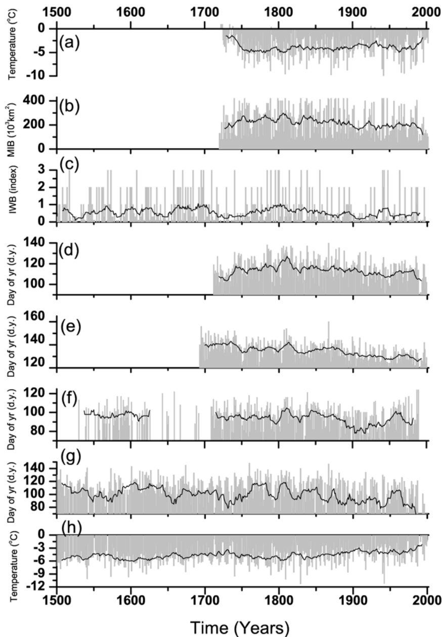
Figure 2 Time series used in the analysis: (a) Uppsala winter air temperature, (b) maximum annual ice cover extent in the Baltic Sea (MIB), (c) ice winter severity in the Western Baltic (IWB). Day of yr (d.y.) for ice break-up in (d) Lake Mälaren, (e) Torneå River, (f) port of Riga, and (g) port of Tallinn. Panel (h) shows winter air temperature in Tallinn.
