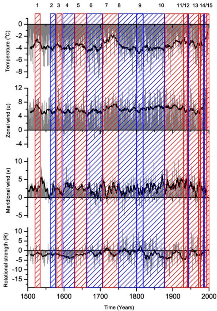
Figure 12 Gray bars show seasonal winter data from the two gridded data sets (Table 1 columns i and j): (top) Baltic Sea mean winter air temperature; (second panel) zonal wind component, westerly winds when positive and easterly winds when negative; (third panel) meridional wind component, southerly winds when positive and northerly winds when negative; and (bottom panel) rotational flows, cyclonic circulation when positive and anti-cyclonic when negative. Black line in all panels is a 15-y running mean. Blue and red field covers time periods classified by matching pursuit (MP) as mild or cold. The number above each field corresponds to the number in Table 2.
