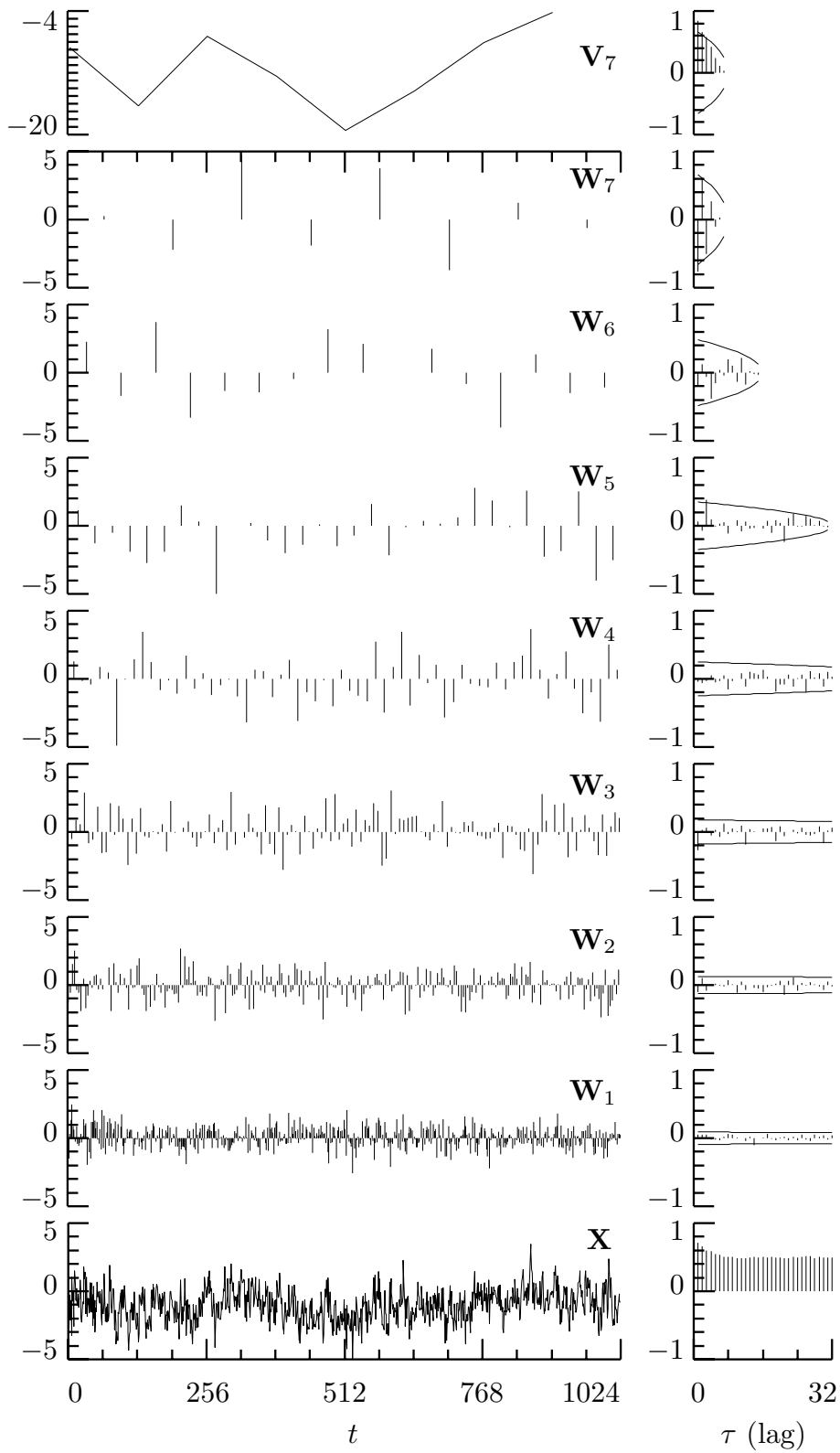
Figure 1. LA(8) DWT coefficients for simulated FD time series with \delta = 0.4 and sample ACSs.
