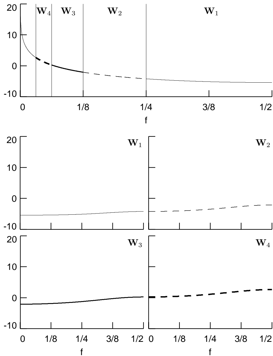
Figure 8. SDFs for FD process with \delta = 0.4 (top) and for LA(8) wavelet coefficients W_1 , W_2 , W_3 and W_4 (vertical axes are in measured in decibels).
