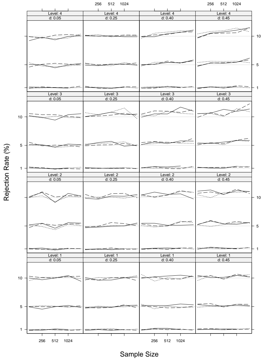
Figure 9. Rejection rates for FD processes using white noise critical levels, N = 128, 256, 512, 1024 and 2048 . The solid line is the Haar wavelet filter, the dotted line is the D(4) and the dashed line is the LA(8) . Each cell corresponds to a different combination of the level j of the DWT and long memory parameter \delta . The rows correspond to – from bottom to top – levels 1, 2, 3 and 4, and the columns correspond to – from left to right – \delta = 0.05, 0.25, 0.40 and 0.45 .
