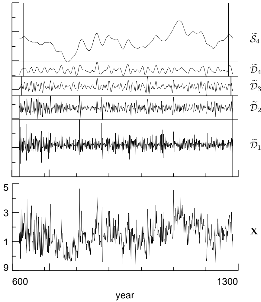
Figure 2. Level J_0 = 4 MODWT multiresolution analysis of Nile River minima (in meters) using the Haar wavelet filter.
