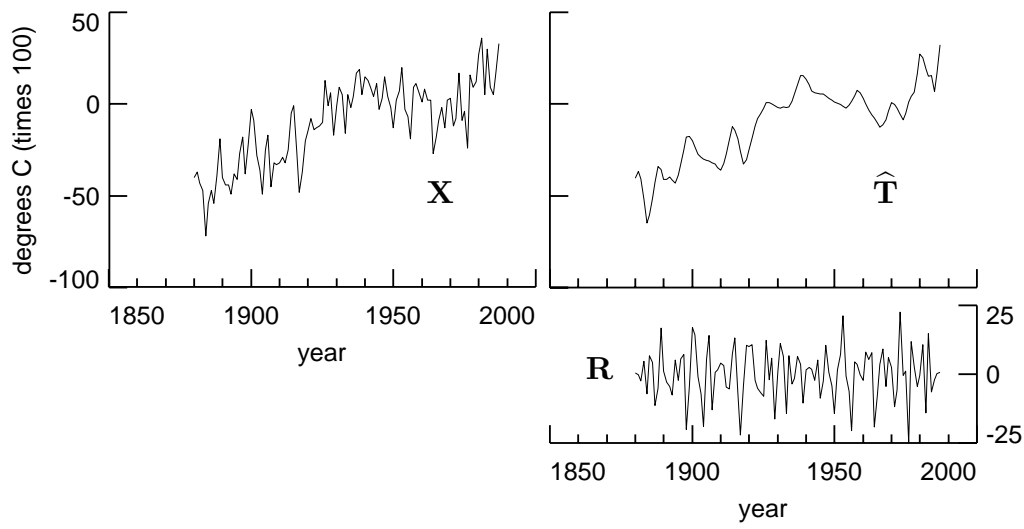
Figure 13. Decomposition of Hansen–Lebedeff global temperature index into trend \hat{\mathbf{T}} and residuals \mathbf{R} \equiv \mathbf{X} - \hat{\mathbf{T}} . The time series \mathbf{X} consists of N = 108 values, and we have used a J_0 = 2 partial DWT based upon the LA(8) wavelet filter (this filter is capable of handling polynomial trends up to order r = 3 ).
