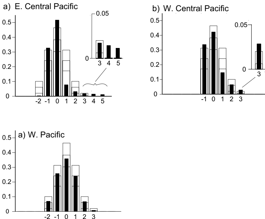
Figure 4: Distributions of monthly-average index values. Bin spacing is 1\sigma . Hash marks at expected value and p=0.05 , p=0.95 levels for a Gaussian-distributed variable with mean and \sigma equivalent to observations.
