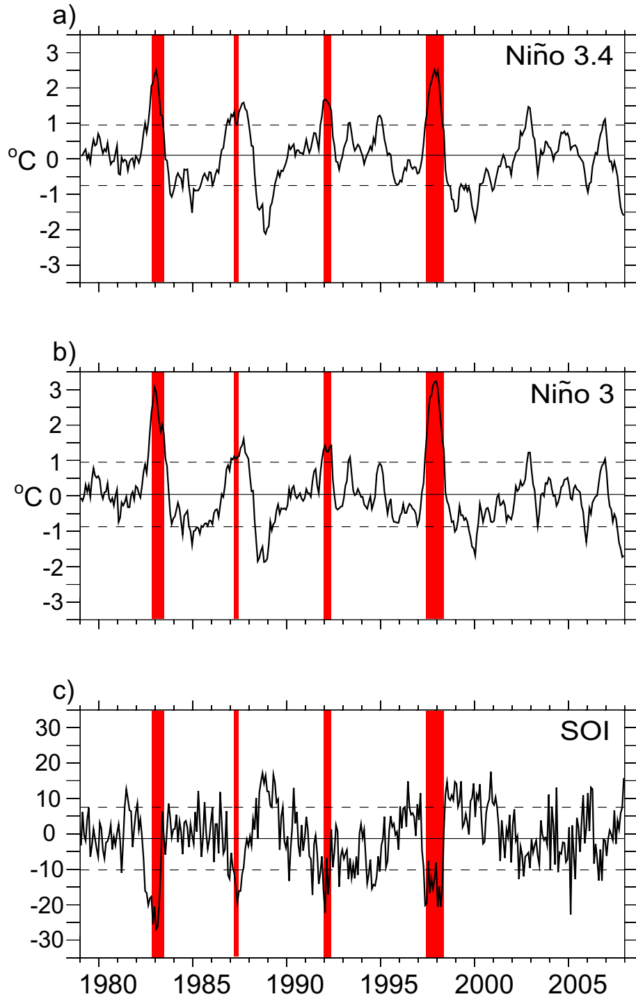
Figure 2: Tropical Pacific SST and SLP based ENSO indices.
