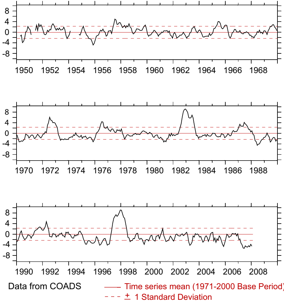
Figure 13: Bjerknes ENSO Index-3. (See Larkin and Harrison 1998.)
