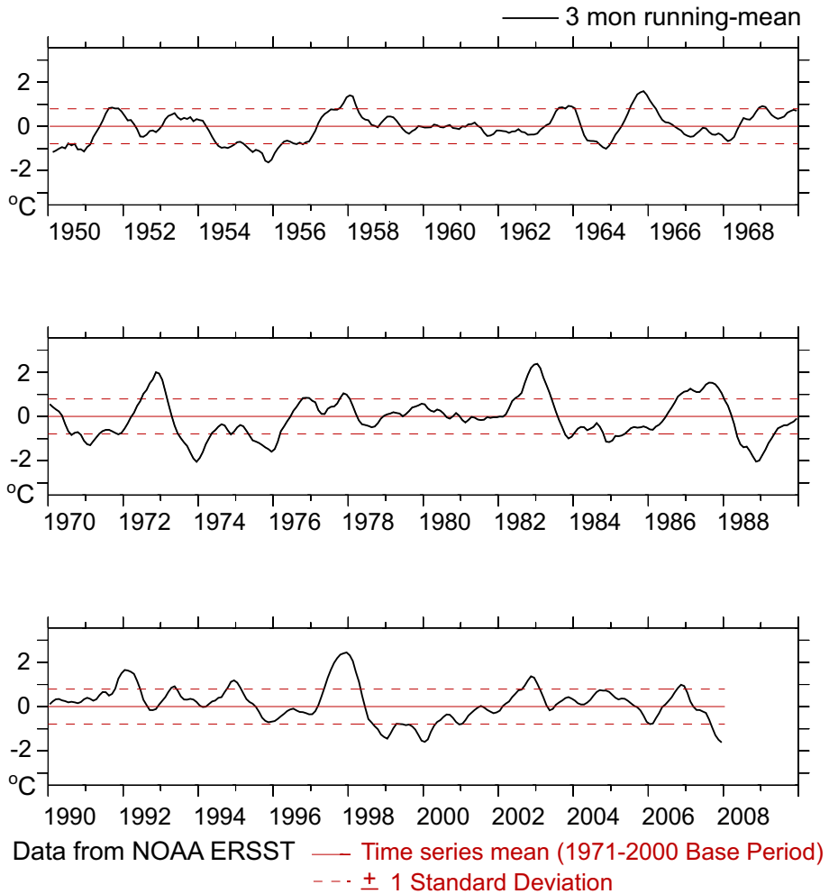
Figure 9: 3-month running mean Niño 3.4 region SSTA. Data from HadISST.
