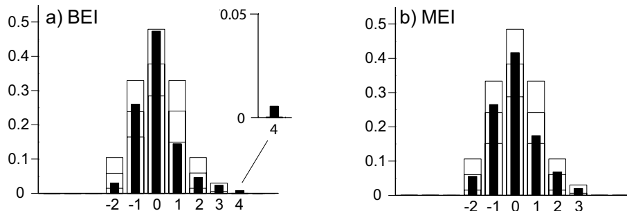
Figure 6: Same as in Fig. 4, except for indices as listed.
