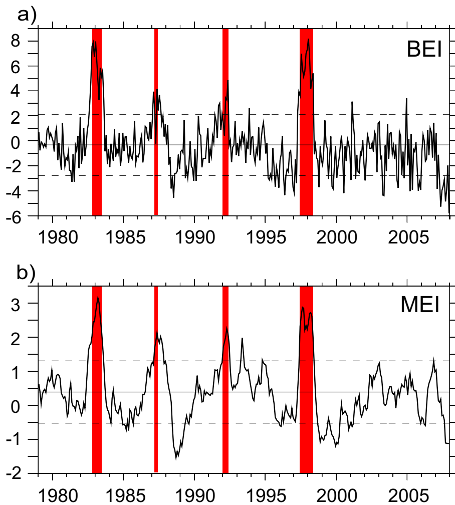
Figure 3: Multivariate ENSO indices (see text.)
